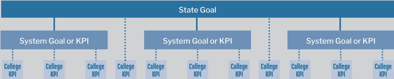
FIGURE 4 Contextualized Metrics
